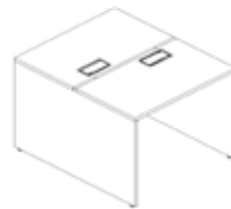
DOUBLE INITIAL WORKSTATION PANEL LEG DEPTH 1400 mm
